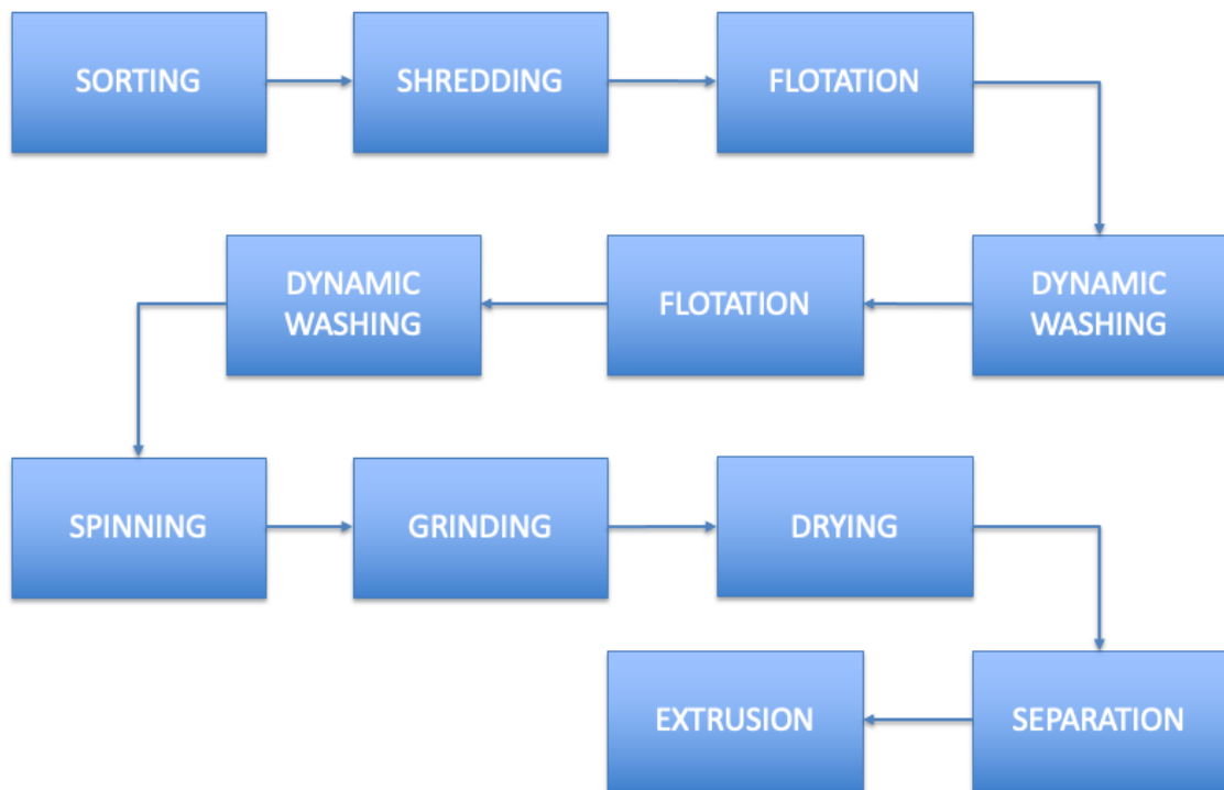
DIAGRAM OF THE LINE FOR RECYCLING OF PLASTICS HAVEL INVESTMENT COMPANY
